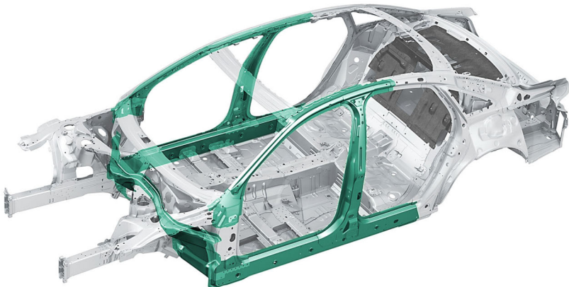
Body with reinforced passenger cell
