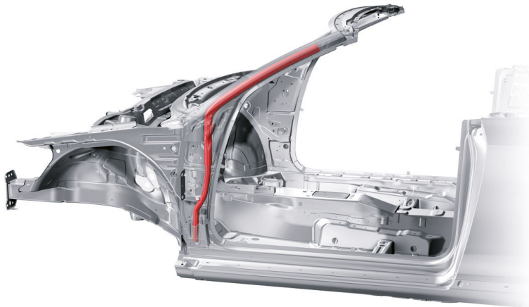
A-pillar reinforcement in the convertible
